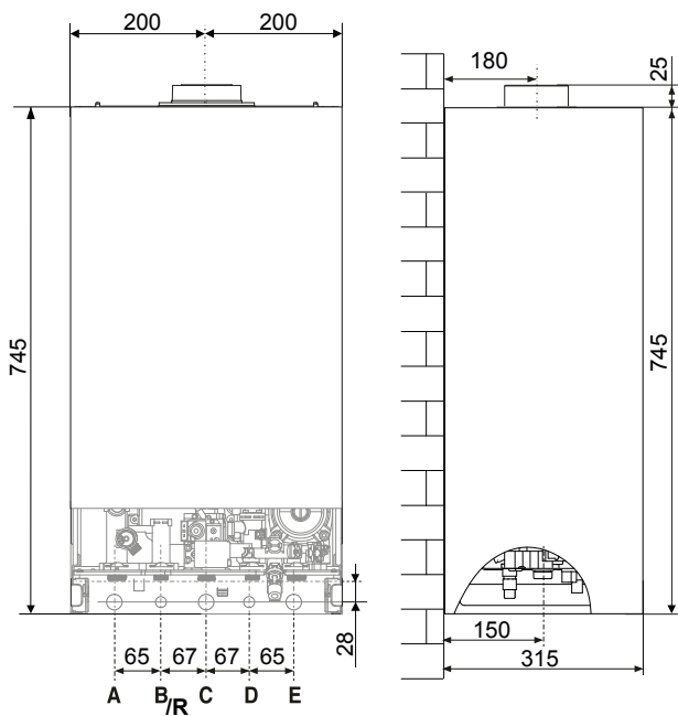
PIGMA ULTRA 25/30 FF PIGMA ULTRA SYSTEM 25/30 FF
