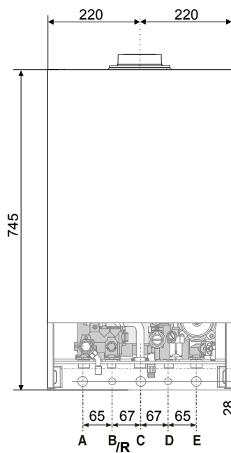
PIGMA ULTRA 35 FF PIGMA ULTRA SYSTEM 35 FF
